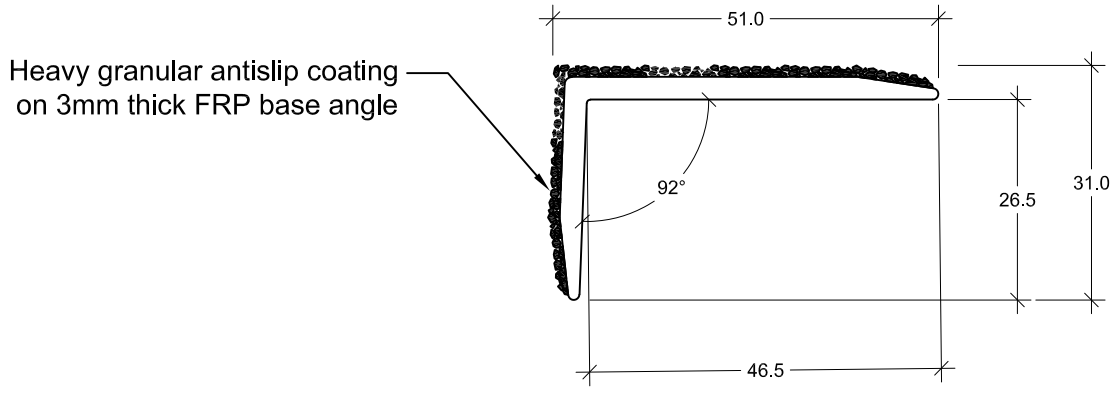
MFRP 50mm profile cross section
