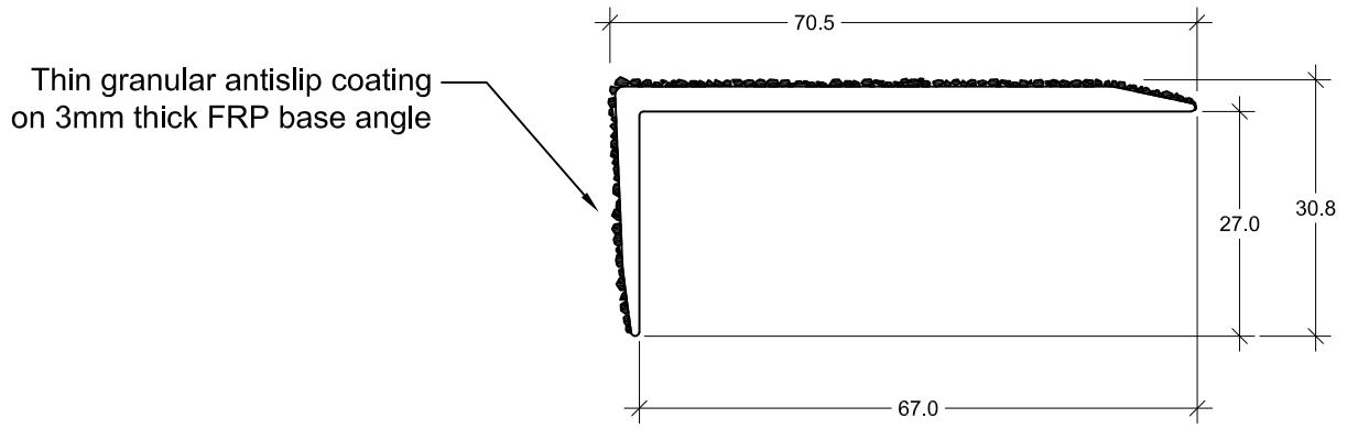
MFRP 70mm profile cross section
