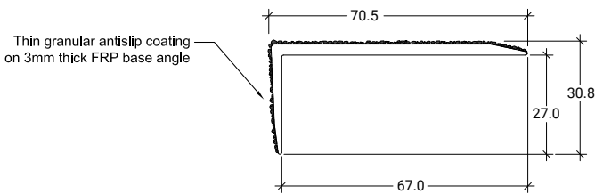
MFRP 70mm profile cross section
